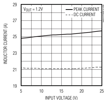
MAXIMUM INDUCTOR CURRENT vs. INPUT VOLTAGE
