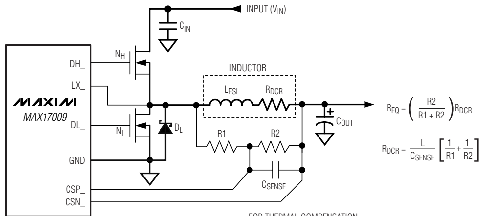
B) OUTPUT INDUCTOR DCR SENSING
