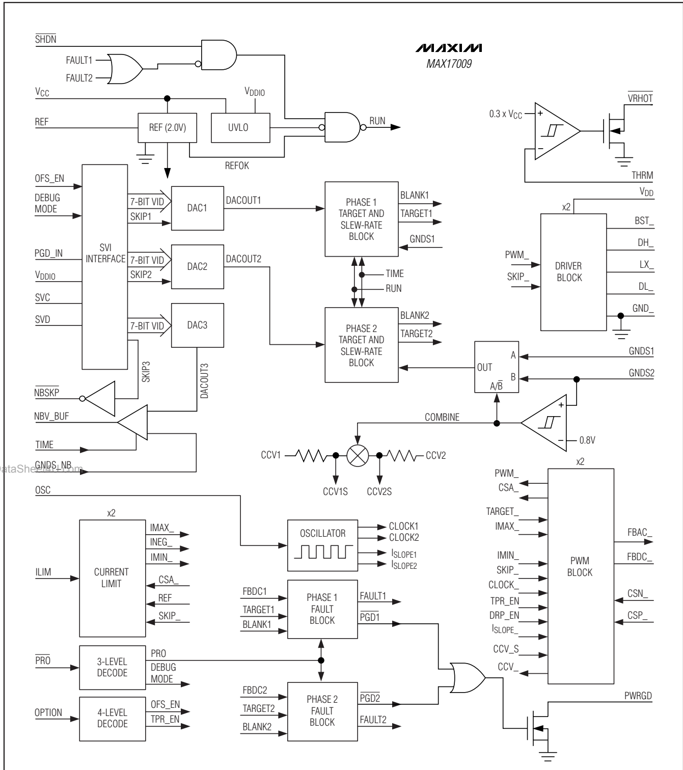
Figure 3. Functional Diagram
