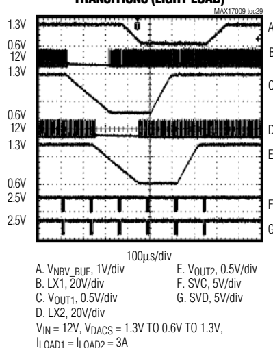
DYNAMIC OUTPUT-VOLTAGE TRANSITIONS (LIGHT LOAD)
