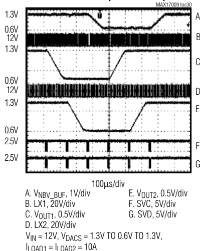
DYNAMIC OUTPUT-VOLTAGE TRANSITIONS (HEAVY LOAD)
