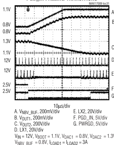
PGD_IN FALLING TRANSITIONS
