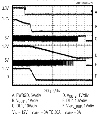
1-PHASE OUTPUT OVERLOAD
