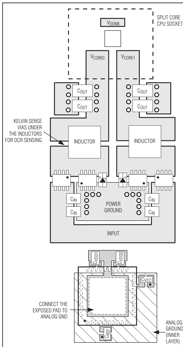
Figure 13. PCB Layout Example
