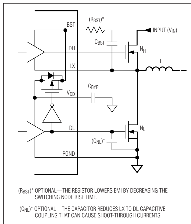
Figure 9. Gate Drive Circuit
