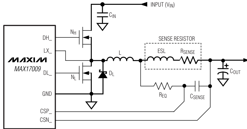
A) SERIES SENSE-RESISTOR SENSING
