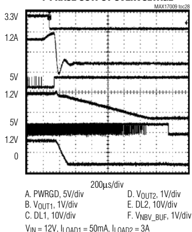
1-PHASE OUTPUT OVERVOLTAGE
