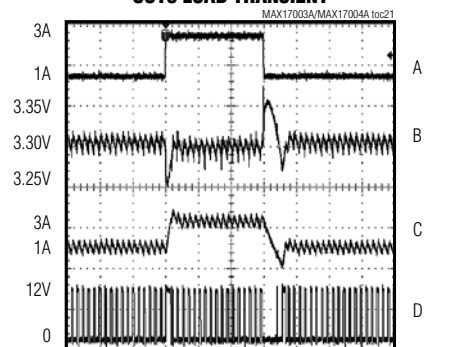
OUT3 LOAD TRANSIENT
