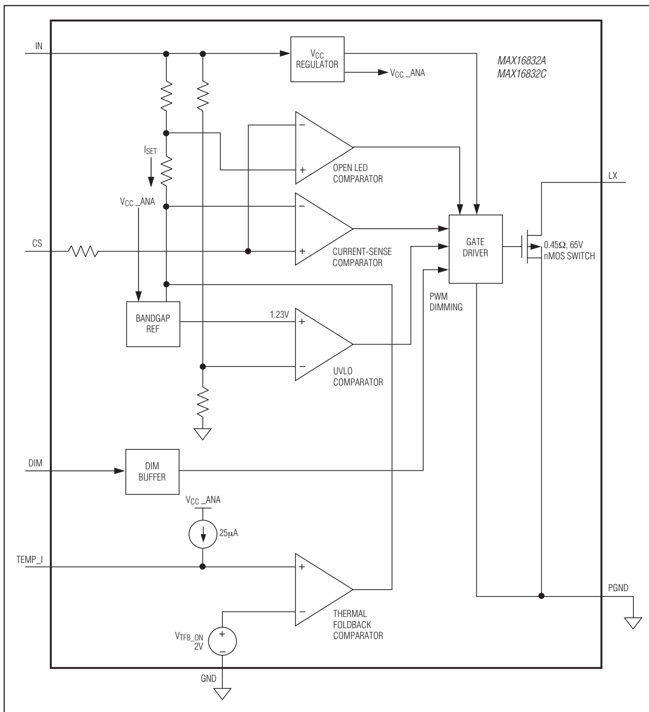
Figure 1. Functional Diagram
