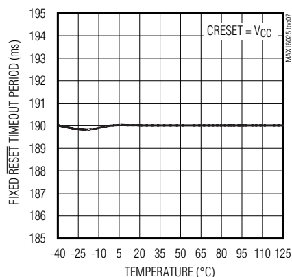
FIXED RESET TIMEOUT PERIOD vs. TEMPERATURE
