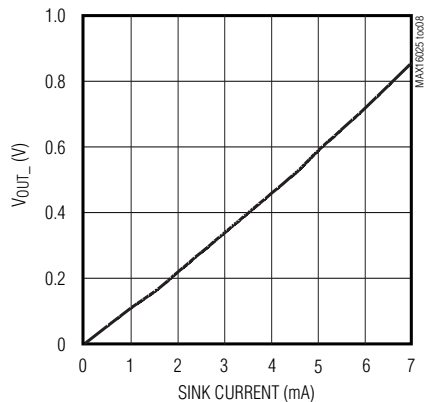
OUT_ LOW VOLTAGE vs. SINK CURRENT
