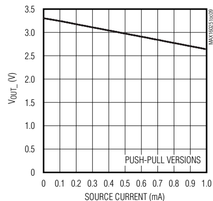
OUT_ HIGH VOLTAGE vs. SOURCE CURRENT
