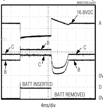
TRANSIENT RESPONSE (BATTERY REMOVAL AND INSERTION)
