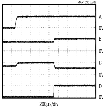
LOAD SWITCH CONTROL (ADAPTER INSERTION)
