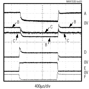
SYSTEM LOAD TRANSIENT
