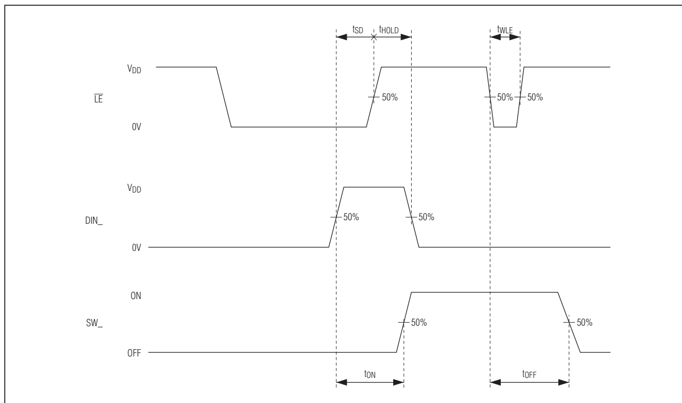
Figure 2. Digital Control ( \overline{DIN1}/\overline{DIN2}/\overline{LE} ) Timing
