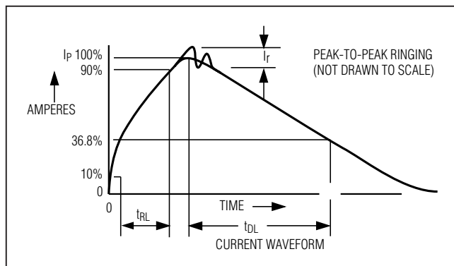
Figure 4. Human Body Model Current Waveform
