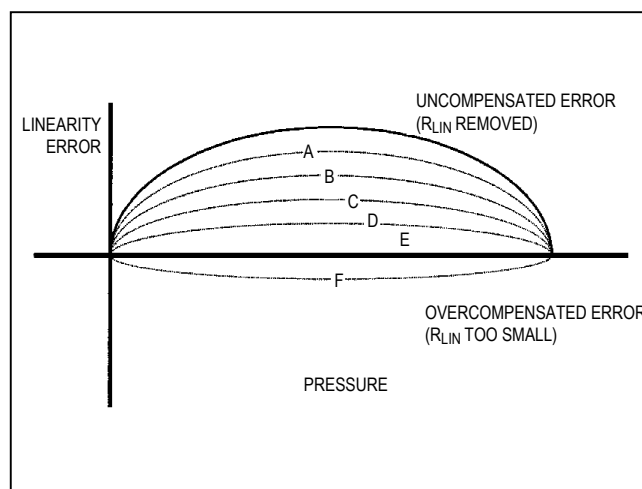
Figure 5. Effect of R_{\text{LIN}} on Linearity Corrections
