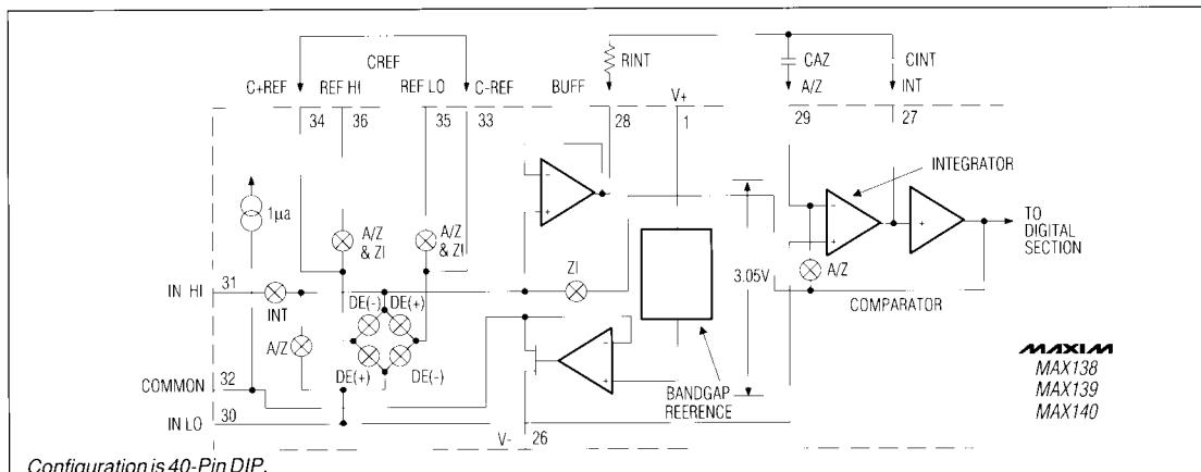
Figure 3. Analog Section of MAX138/139/140
