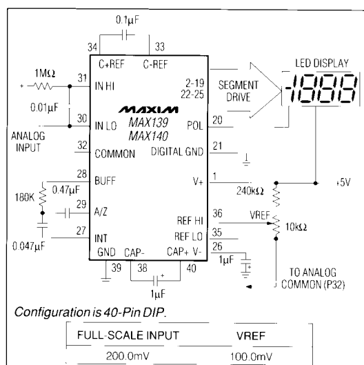
Figure 2. MAX139/MAX140 Typical Operating Circuit
