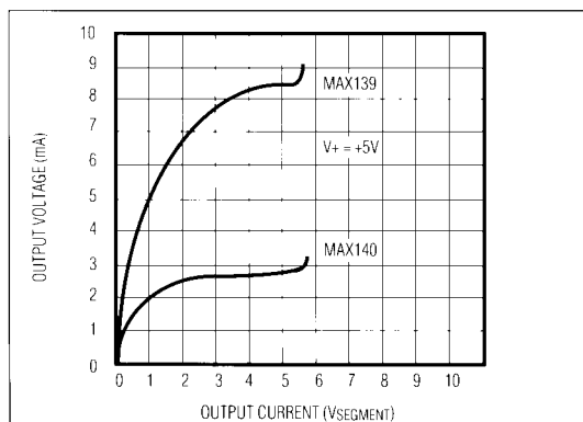
Figure 5. Output Current vs. Output Voltage
