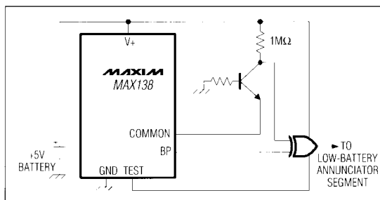
Figure 6. Low-Battery Detector and LCD Segment Drive
