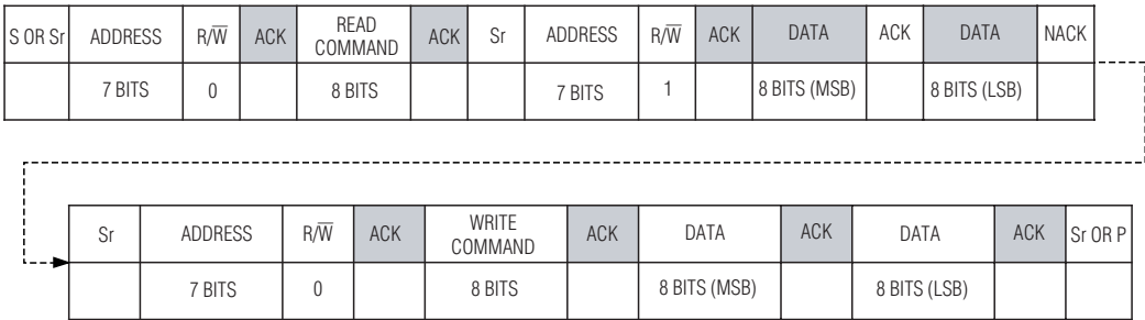
Figure 13. Read-Modify-Write Sequence
