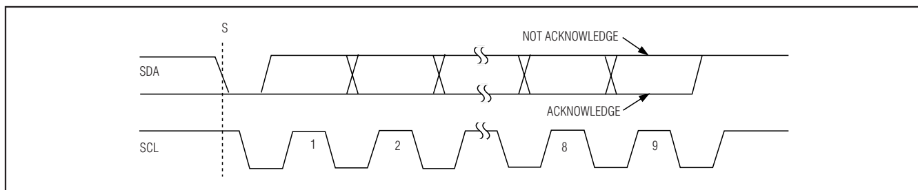
Figure 20. Acknowledge Bits
