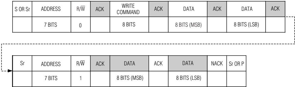
Figure 12. Write/Readback Sequence
