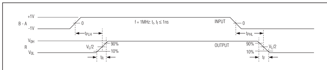
Figure 7. V.11 Receiver Propagation Delays
