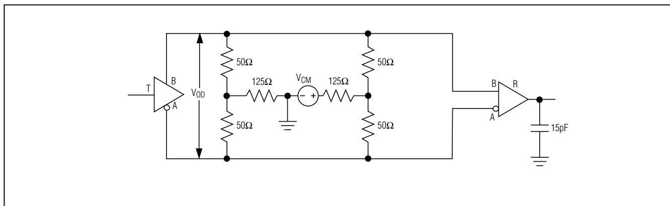
Figure 3. V.35 Transmitter/Receiver Test Circuit
