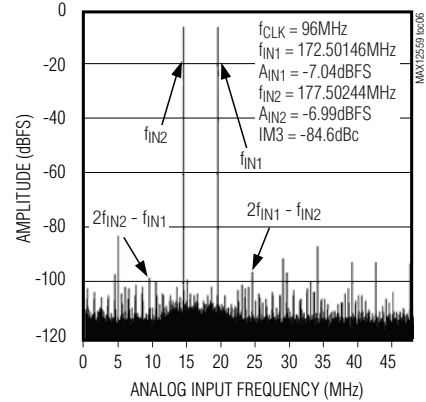
TWO-TONE IMD PLOT (65,536-POINT DATA RECORD)
