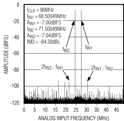
TWO-TONE IMD PLOT (65,536-POINT DATA RECORD)
