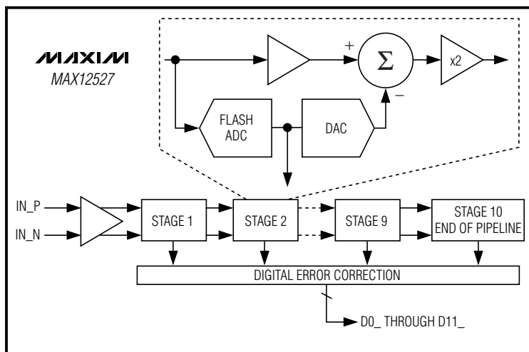
Figure 1. Pipeline Architecture—Stage Blocks
