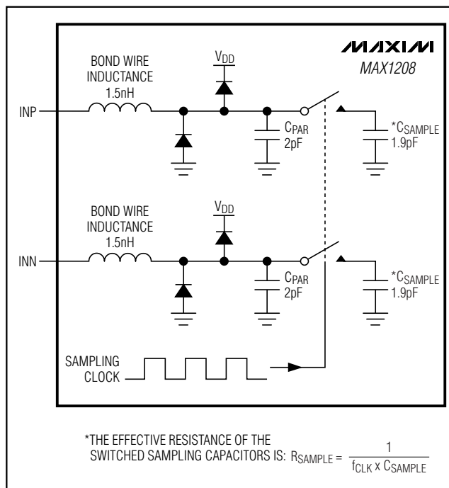
Figure 3. Simplified Input Track-and-Hold Circuit
