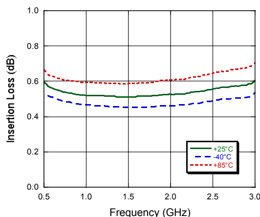
GPS Path Insertion Loss
