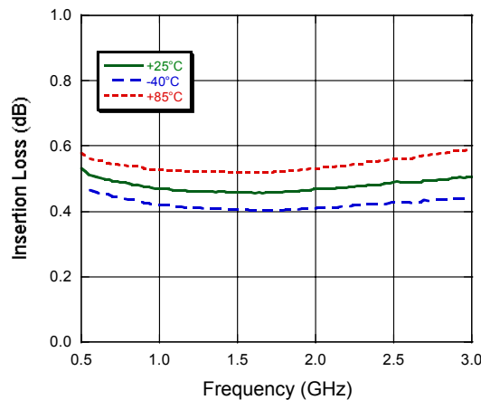
PCS Path Insertion Loss
