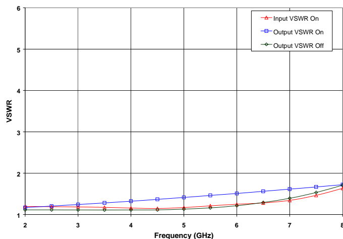
Figure 1. Input and Output VSWR vs. Frequency
