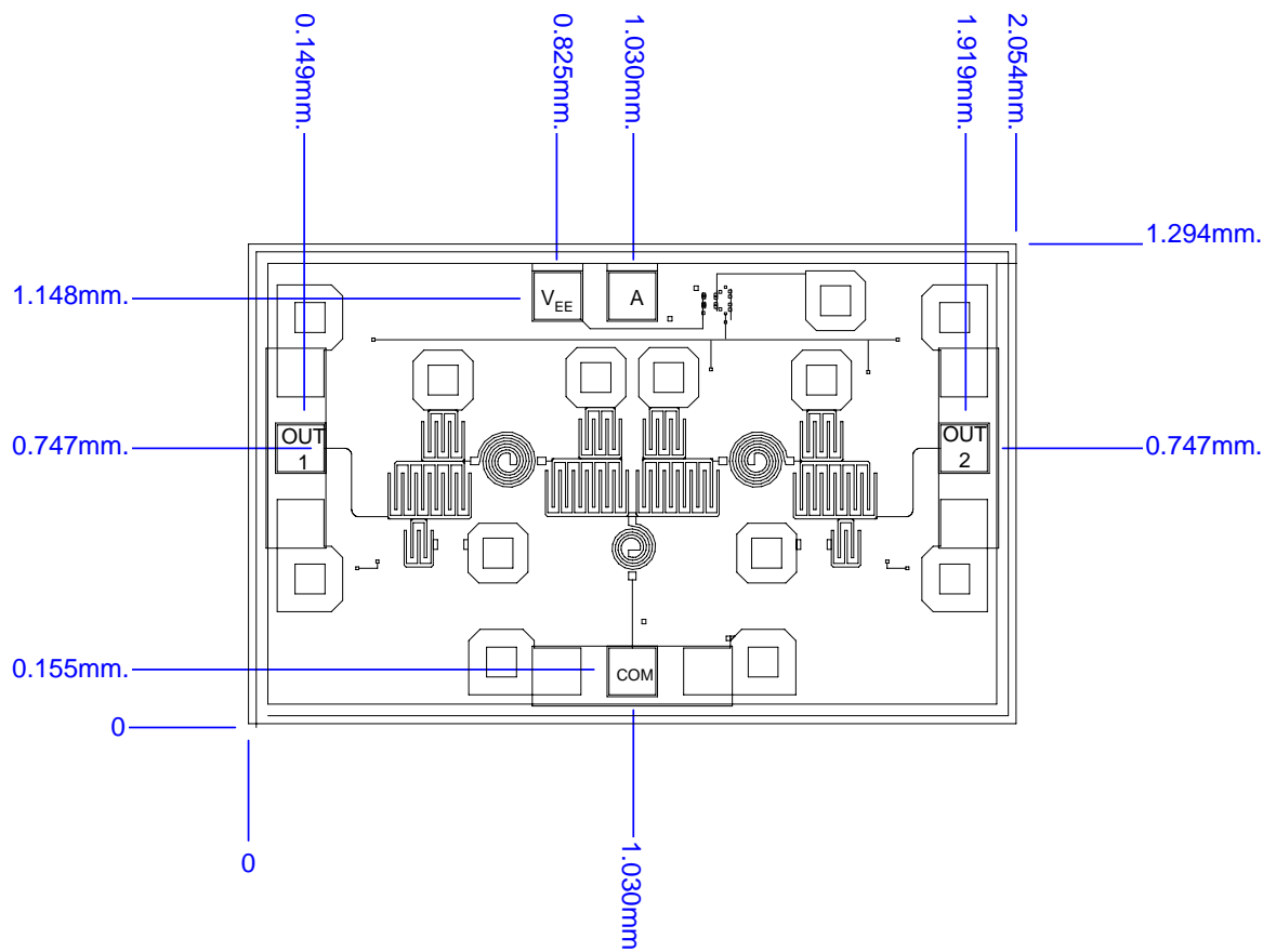
Figure 3. Die Layout
