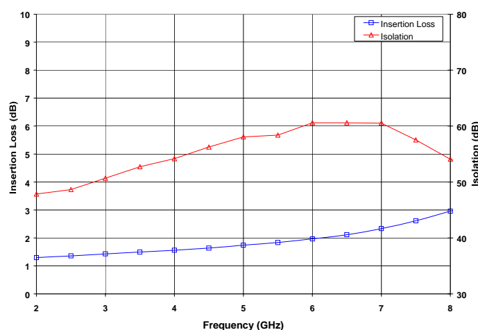
Figure 2. Insertion Loss and Isolation vs. Frequency
