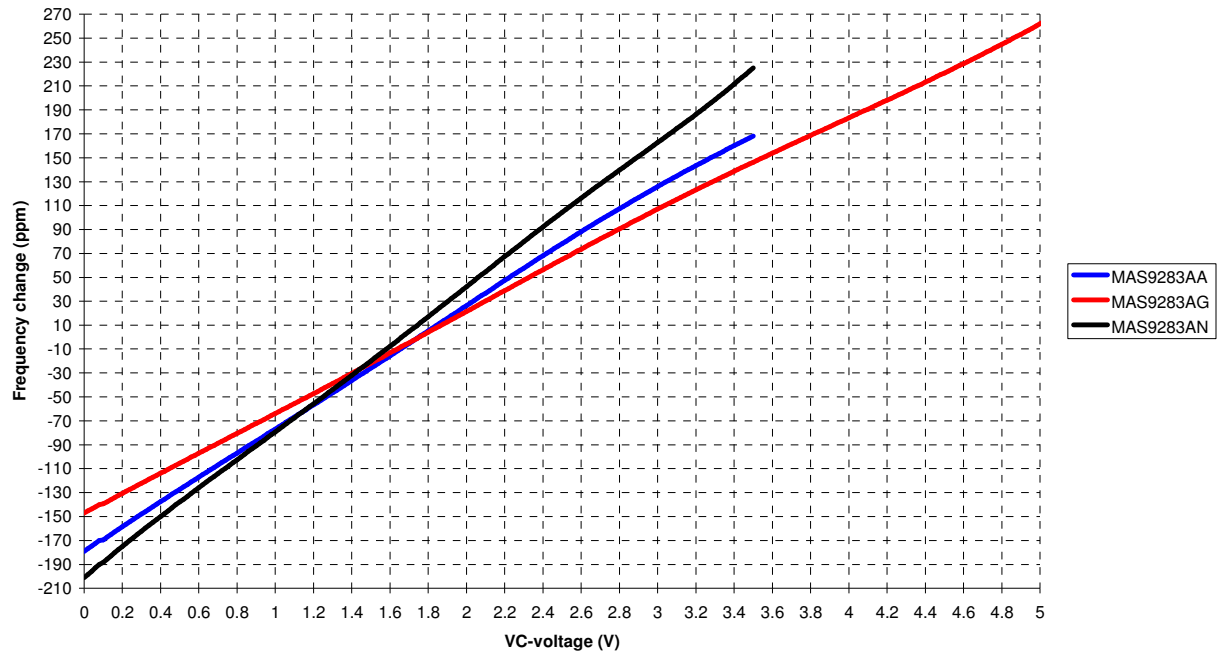
Figure 3. Control voltage sensitivity of MAS9283.
