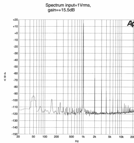
Figure 10. Spectrum, input amplitude 1 Vrms, gain +15.5 dB
