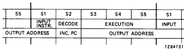
Fig. 11 Instruction cycle.
