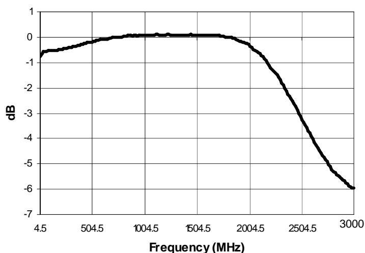
Insertion Loss Port 2 (Pin 4 to Pin 1)
