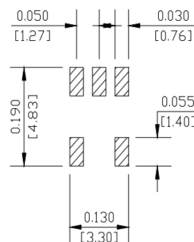
PCB FOOTPRINT
