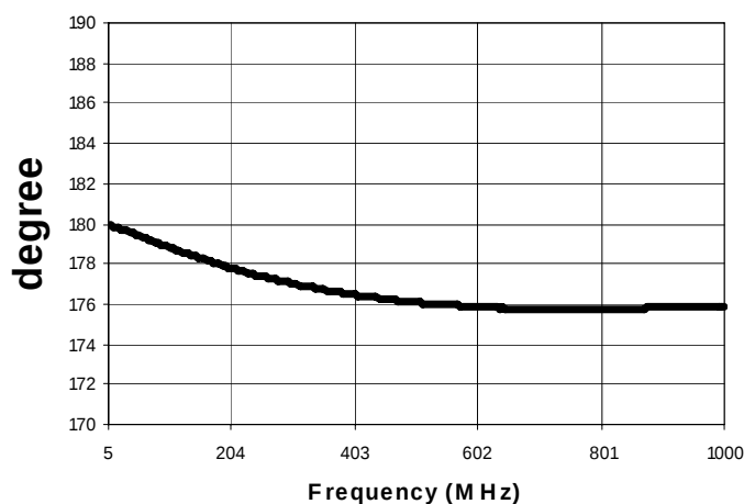
Phase Balance
