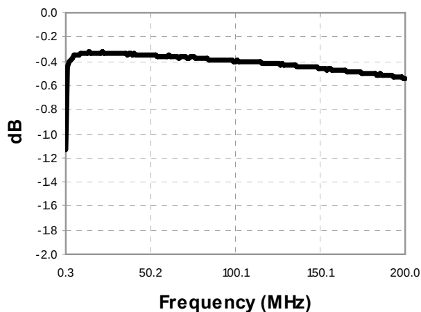
Amplitude Balance
