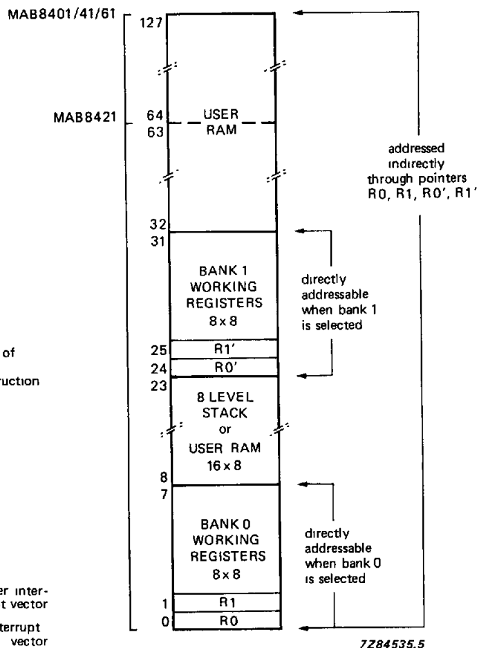
Fig. 6 The data memory map.
