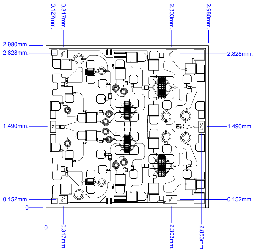
Figure 5. Die Layout
