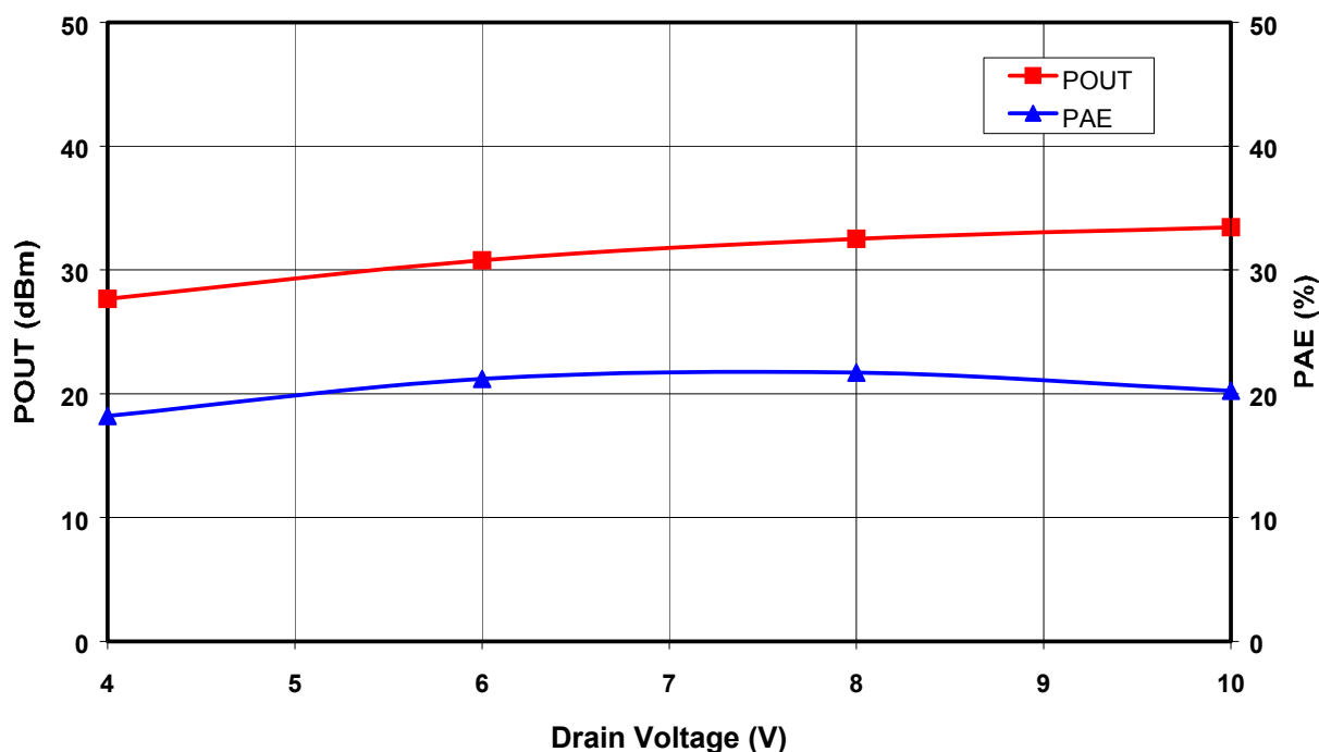
Figure 2. Saturated Output Power and Power Added Efficiency vs. Drain Voltage at f_0 = 10.5 GHz.
