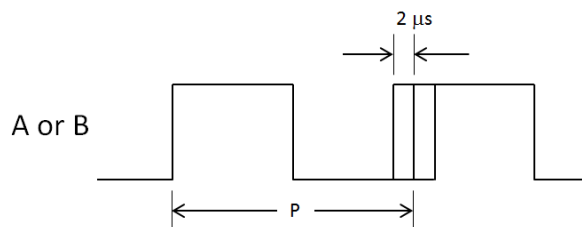
Figure 13: ABZ Jitter
