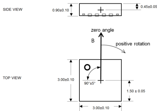
Figure 3: Zero Angle of Unprogrammed MA700
