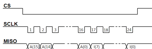
Figure 11: Timing Diagram for SPI Angle + Index Readout
