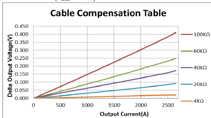
Figure1 Cable Compensation at Various Resistor Divider Values
