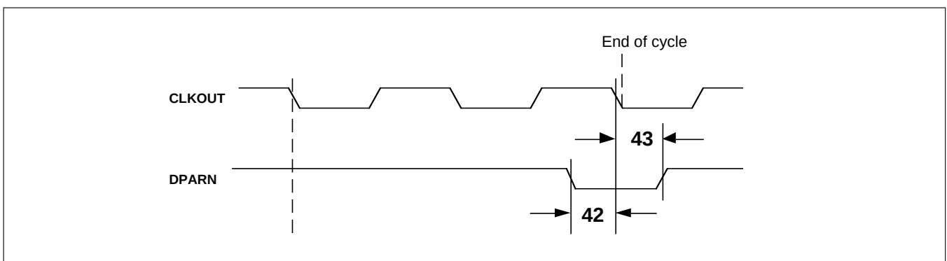
Figure 31: DPARN Timing
