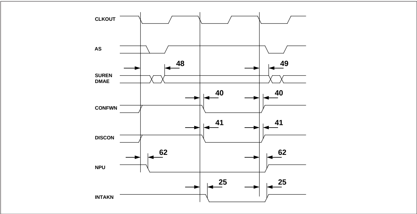
Figure 28: Discrete Timings
