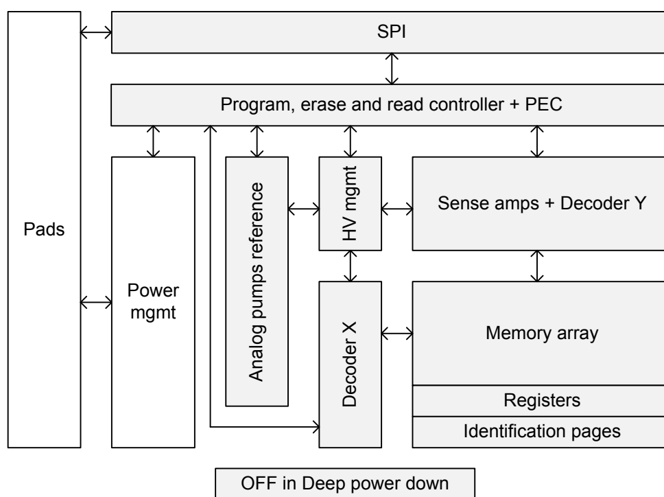
Figure 3. Block diagram
