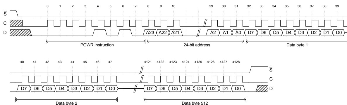
Figure 25. Page write
