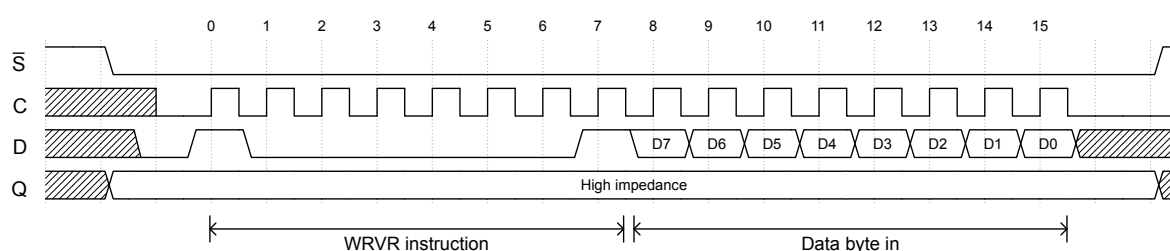
Figure 13. Write volatile register
