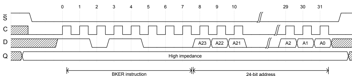
Figure 21. Block erase
