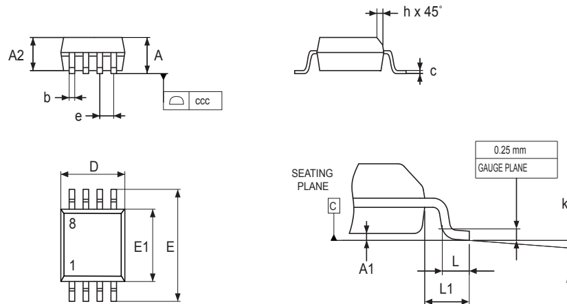
Figure 40. SO8N - Outline
