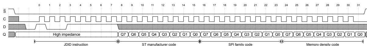
Figure 29. JEDEC identification
