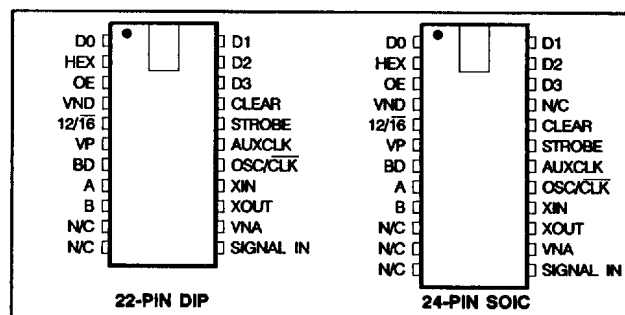
Figure 1 Pin Diagram
