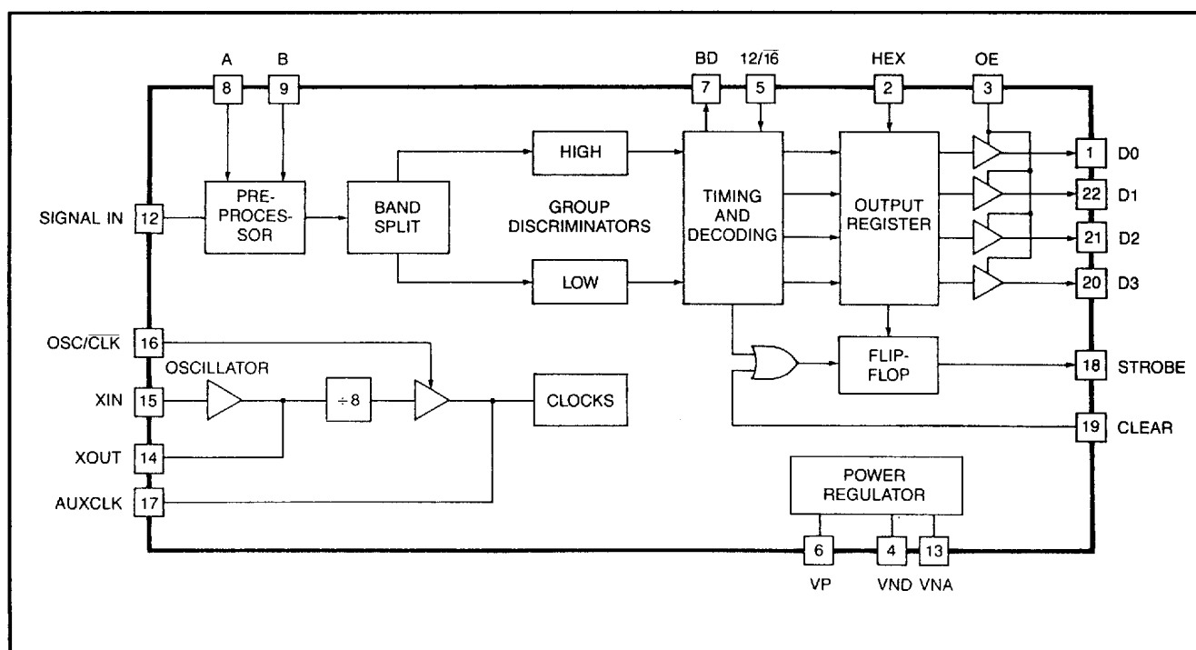
Figure 2 Block Diagram
