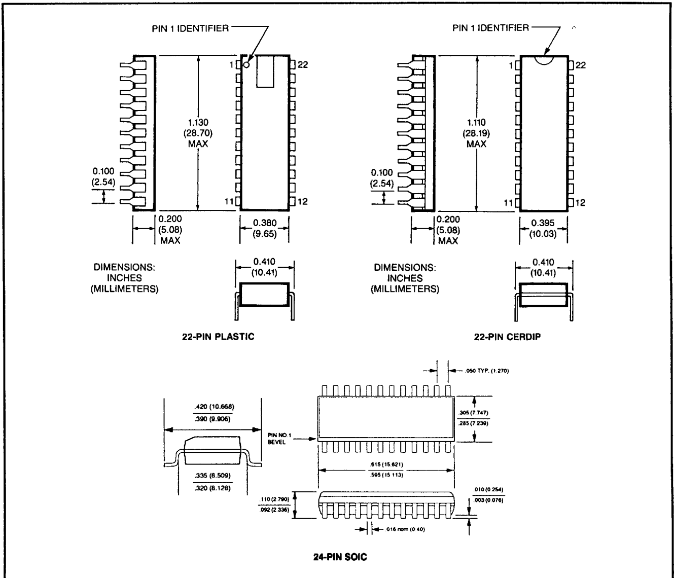
Figure 8 Package Dimensions
