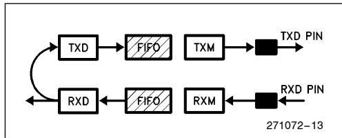
Figure 14. Auto Echo
