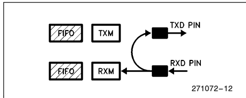
Figure 13. Remote Loopback
