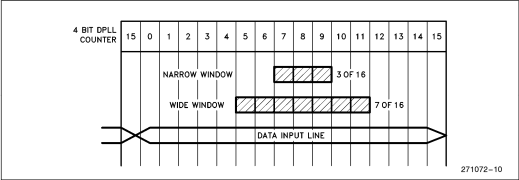
Figure 10. Sampling Windows
