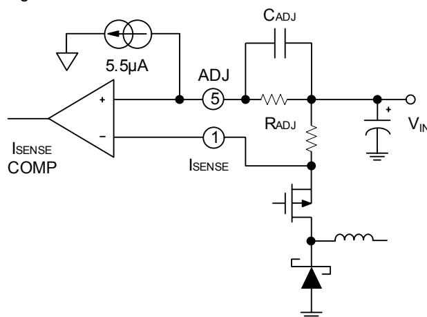
FIGURE 2. Current Sensing by External Resistor
