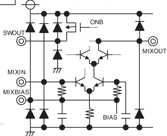
7 MIXIN,MIXB IAS,MIXOUT,SWOUT
