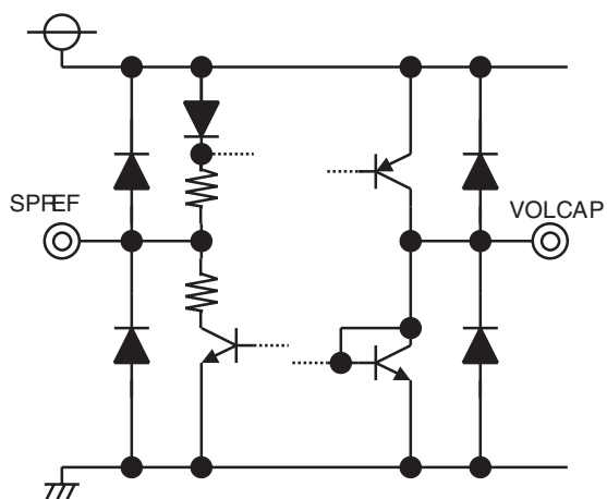
16 SPREF , VOLCAP
