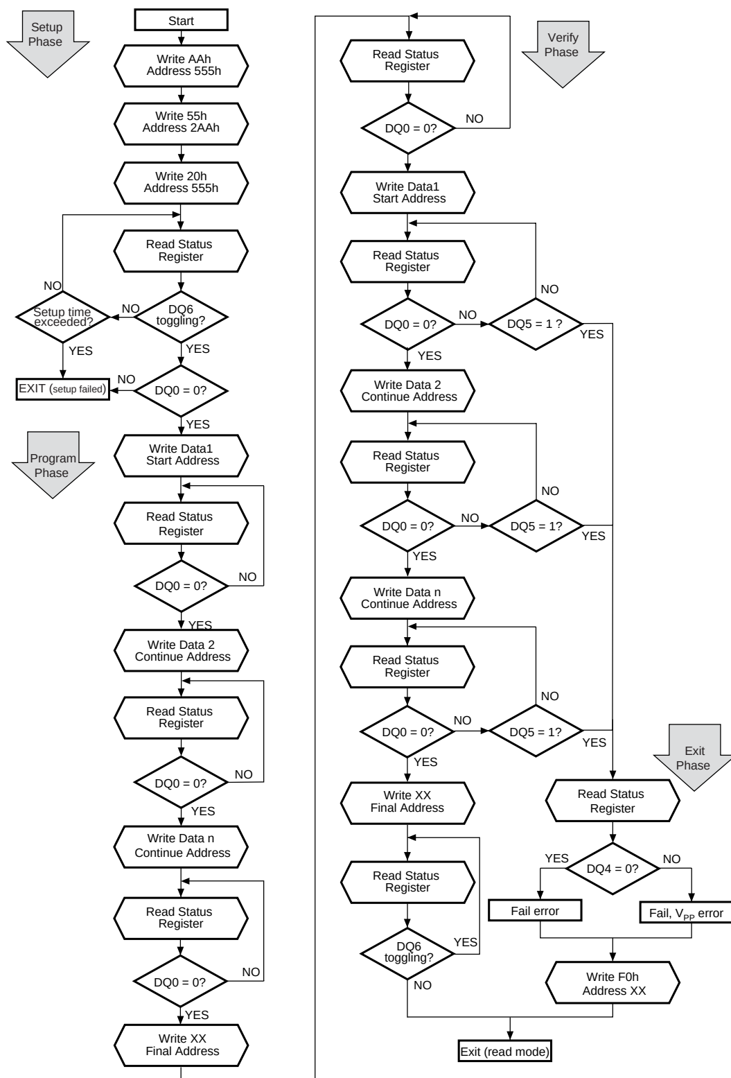
Figure 7. Multiple Word Program Flowchart for 64Mbit Top and Bottom Die
