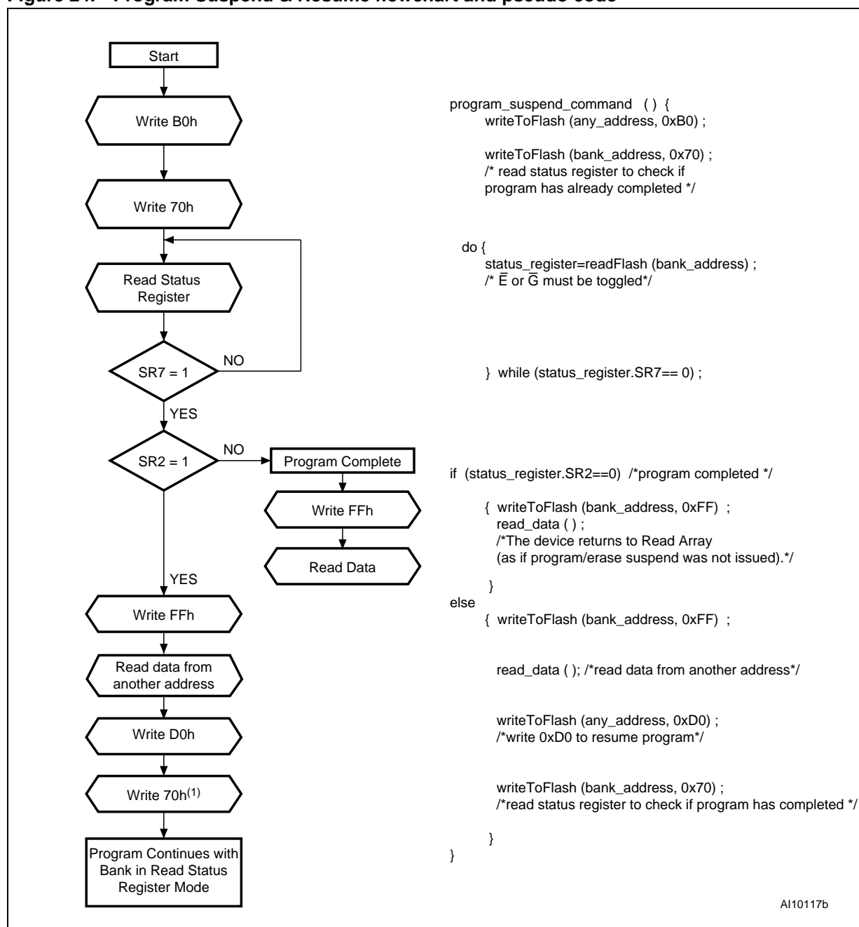
Figure 24. Program Suspend &amp; Resume flowchart and pseudo code
