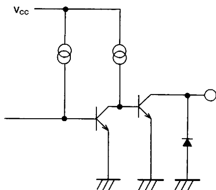
4 Lock Output
