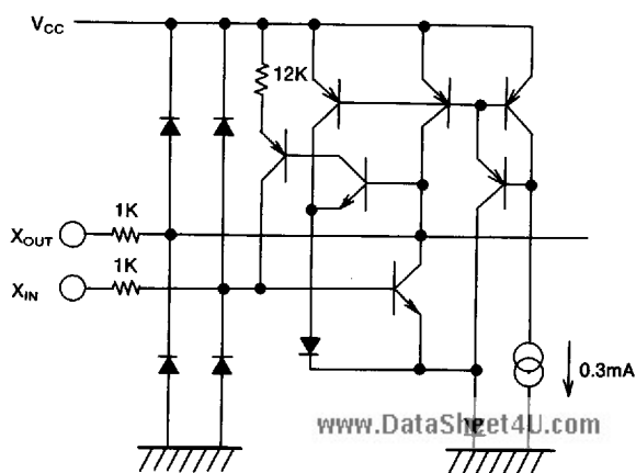
5 OSC Circuit
