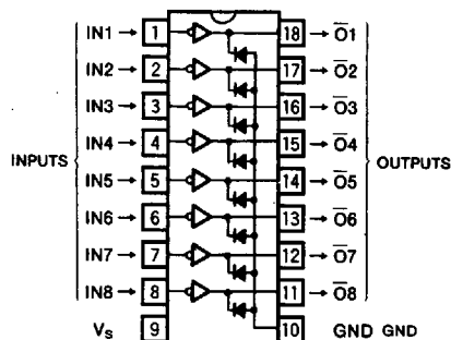
Outline 18P4
