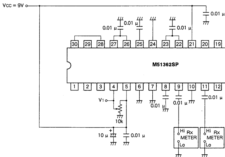
TEST CIRCUIT 2
