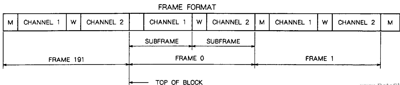
Fig. 6 Timing
