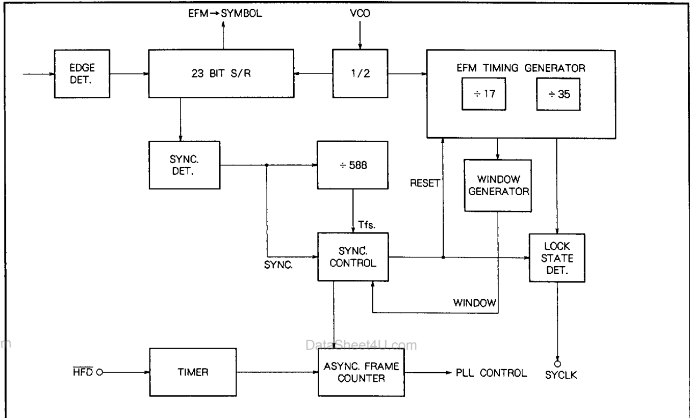
Fig. 1 Frame synchronization block diagram
