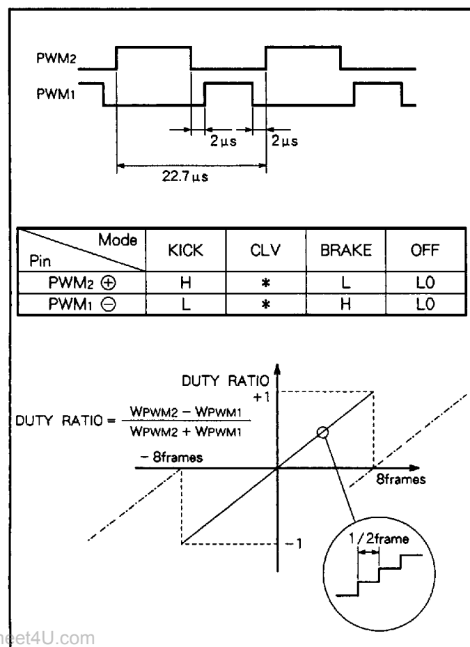
Fig. 7 CLV waveform
