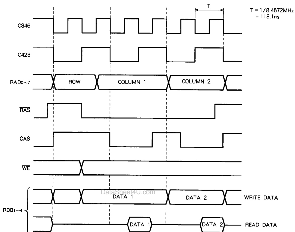
(a) Symbol data/flag, read/write timing
