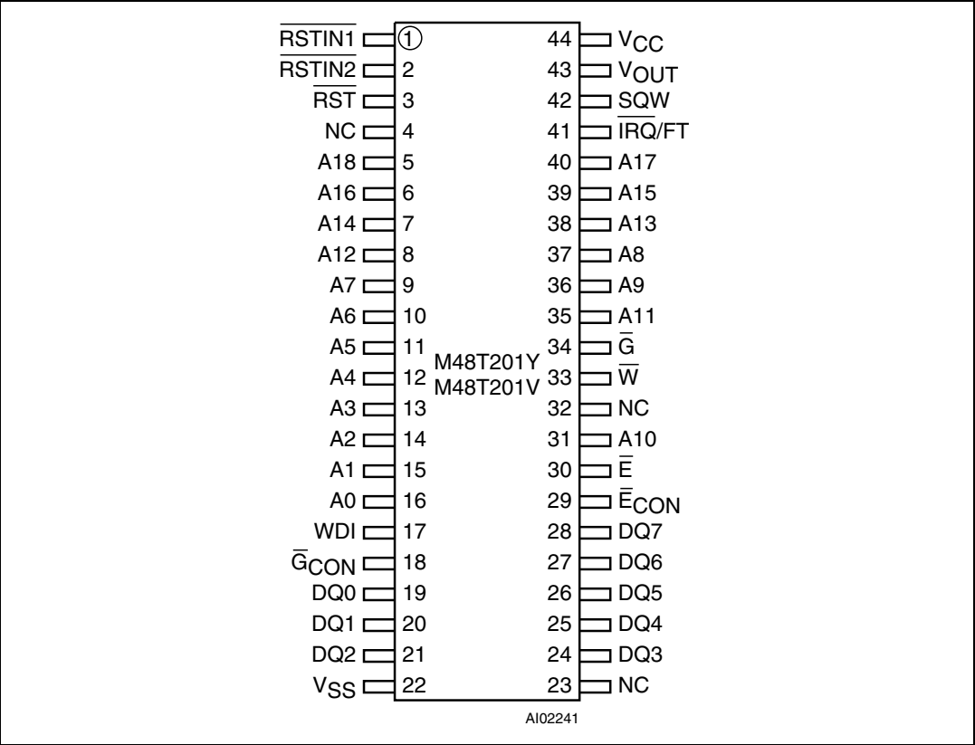
Figure 2. SOIC connections
