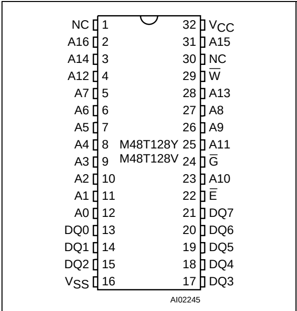
Figure 3. DIP Connections
