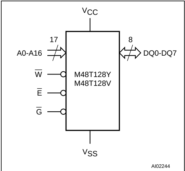
Figure 2. Logic Diagram
