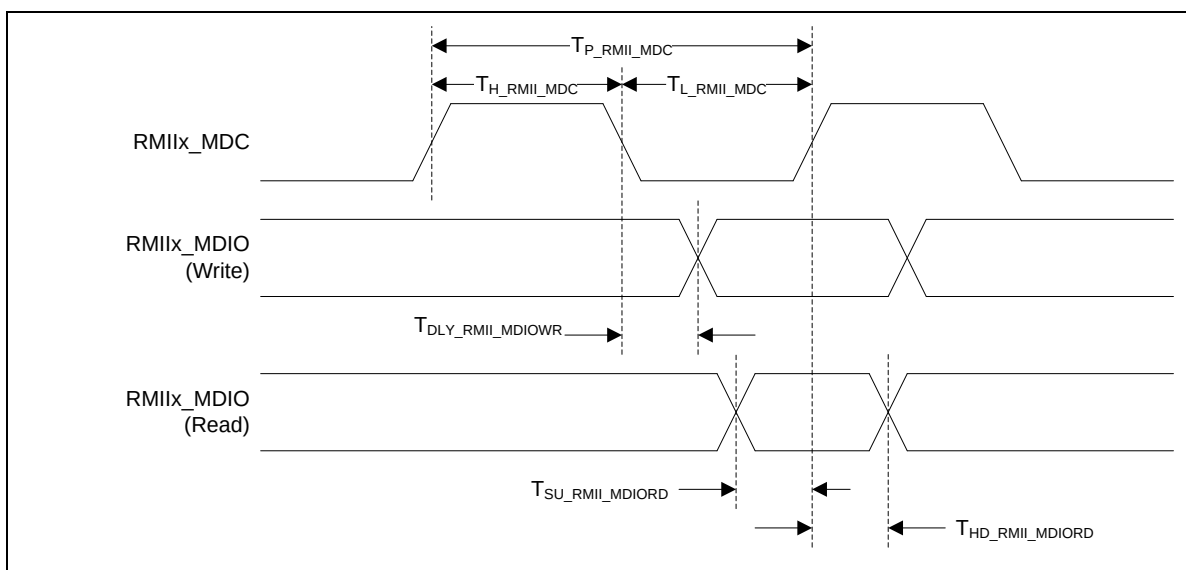
Figure 8.13-2 Ethernet PHY Management Interface Timing Diagram
