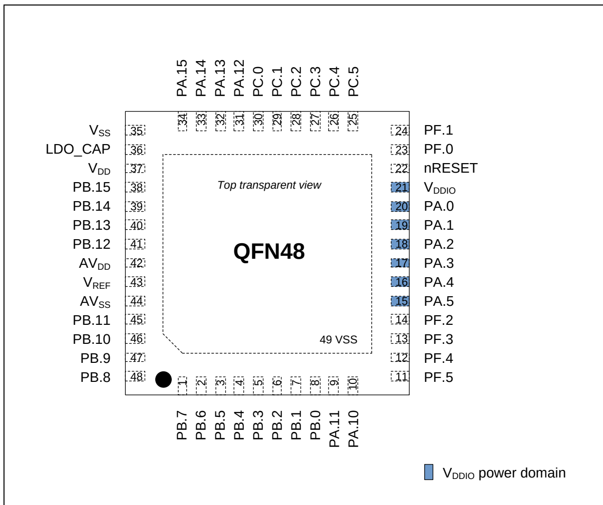
Figure 4.1-2 QFN-48 Pin Diagram
