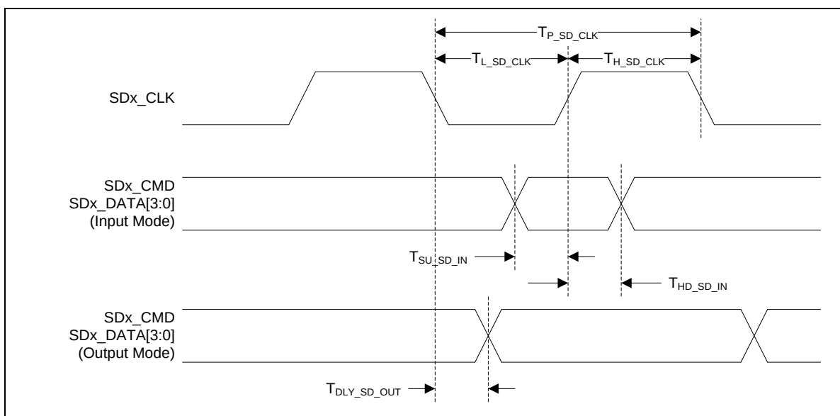
Figure 8.14-1 SDIO Default Mode
