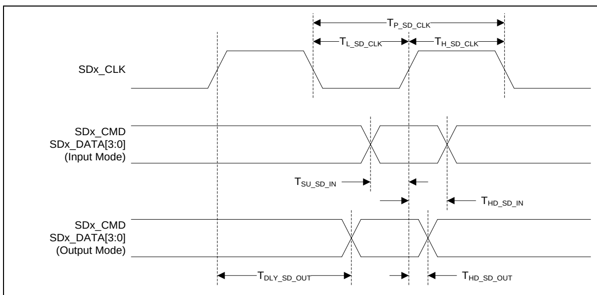
Figure 8.14-2 SDIO High-speed Mode
