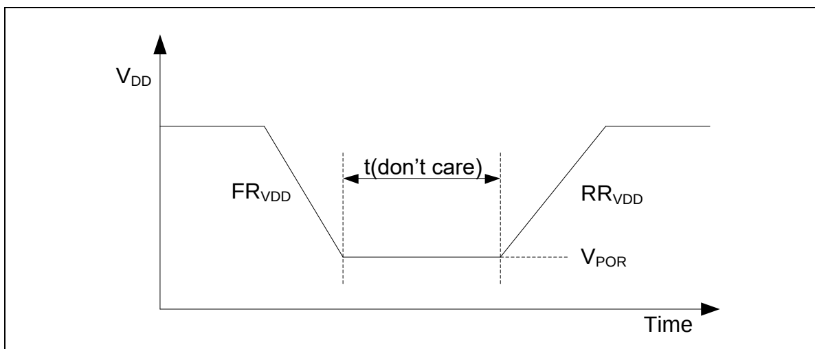
Figure 8.5-1 Power-up Ramp Condition
