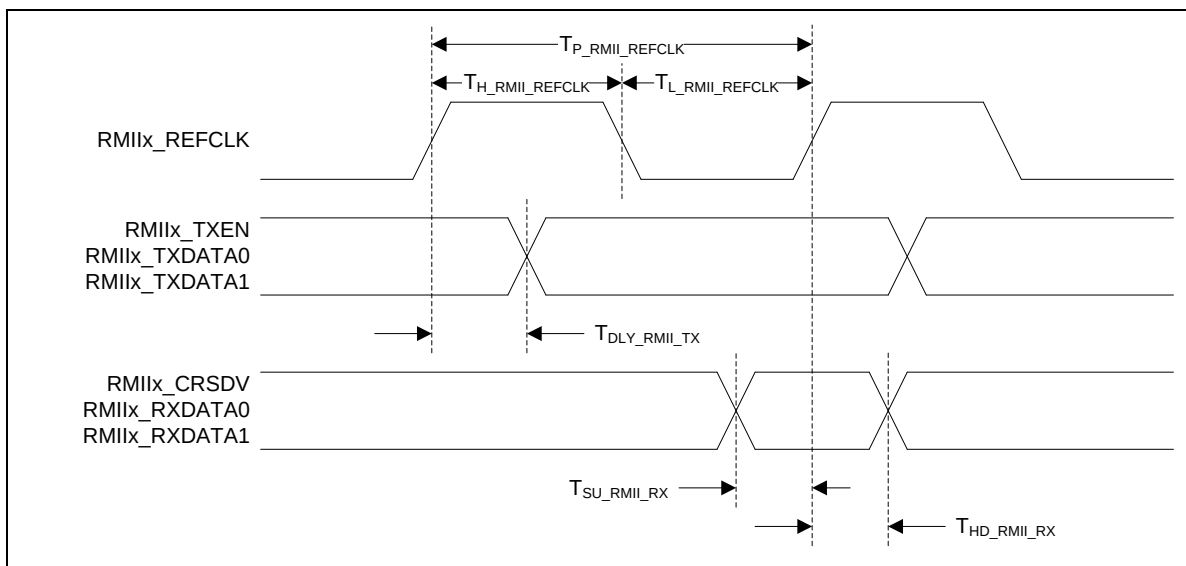
Figure 8.13-1 RMII Interface Timing Diagram
