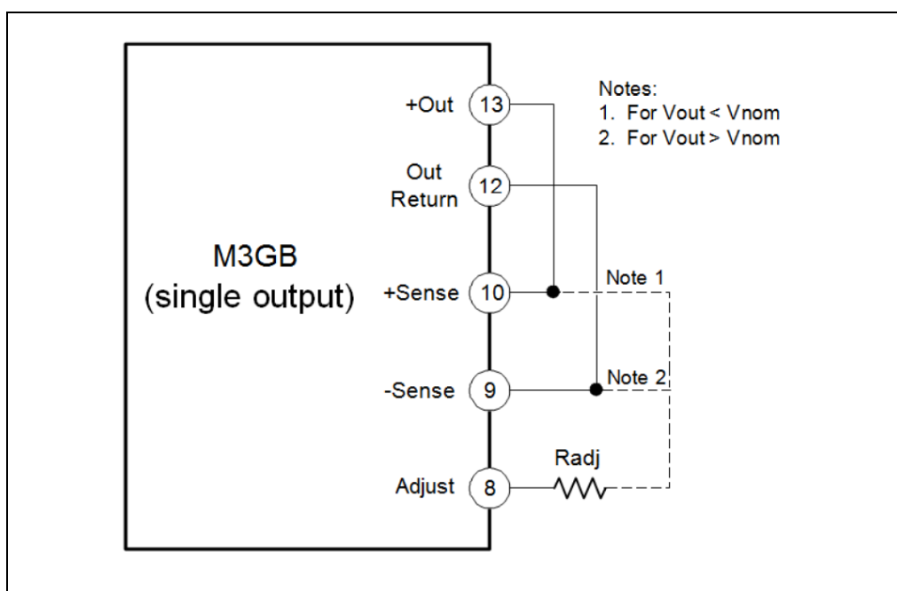
Figure 7 Configuration for Adjusting Single Output Voltage
