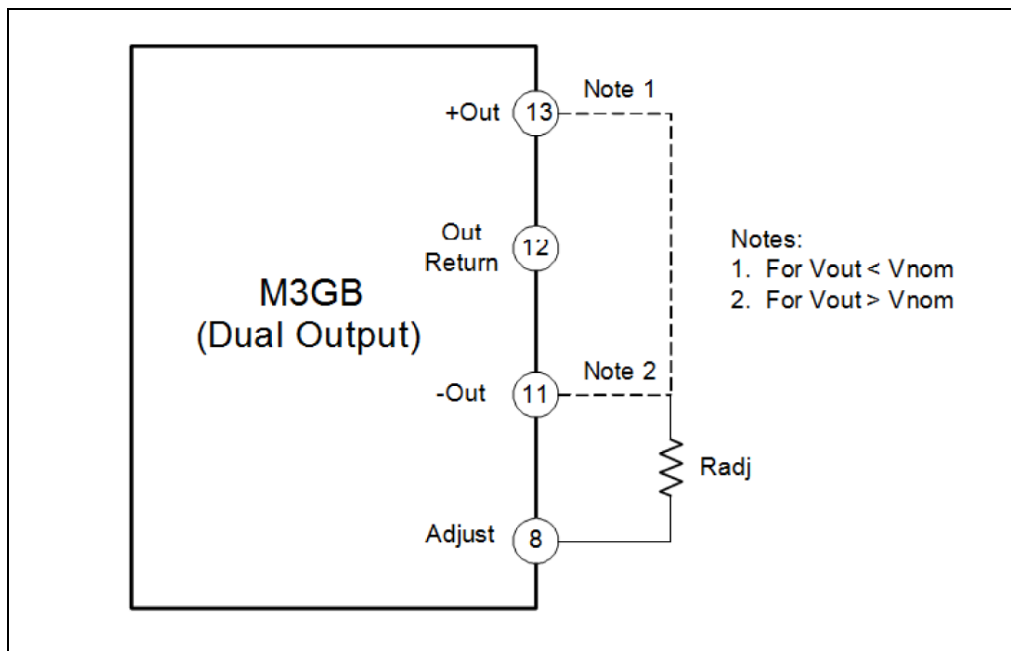
Figure 8 Configuration for Adjusting Dual Output Voltage
