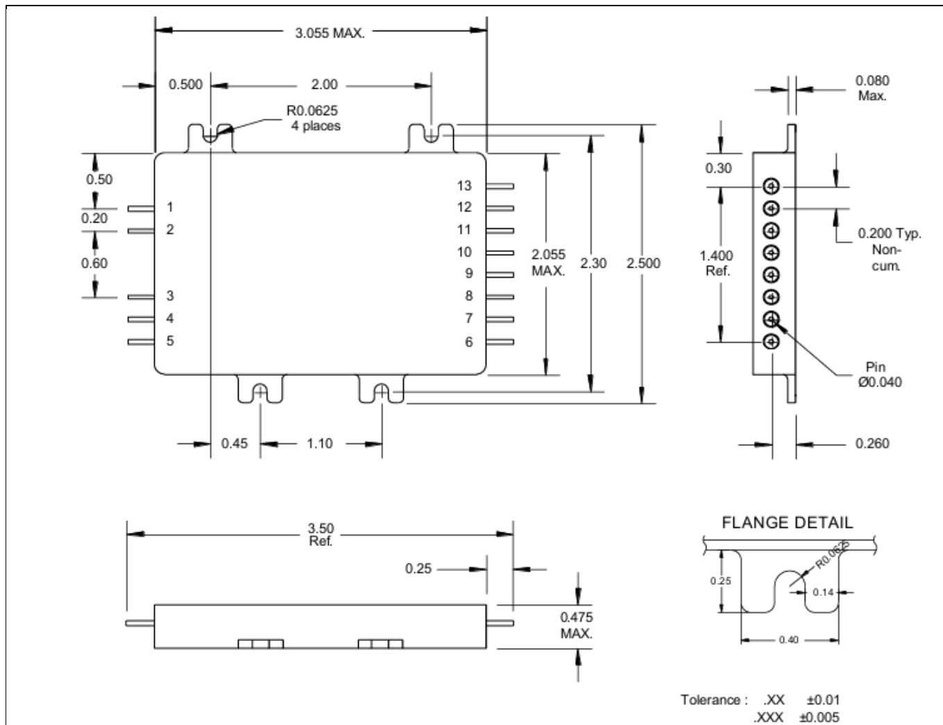
Figure 9 Package outline
