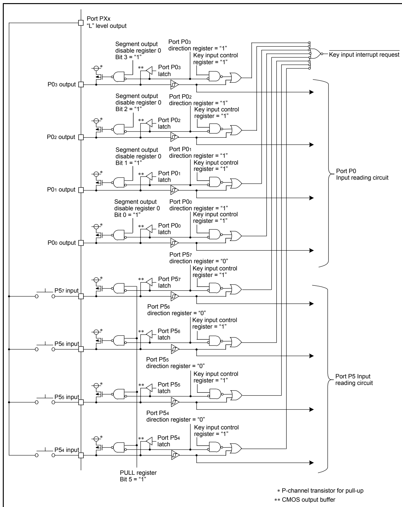
Fig. 21 Connection example when using key input interrupt
