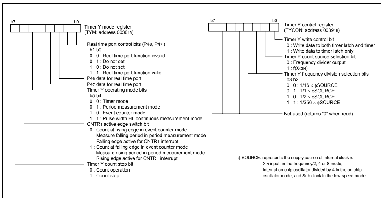
Fig. 30 Structure of timer Y related registers
