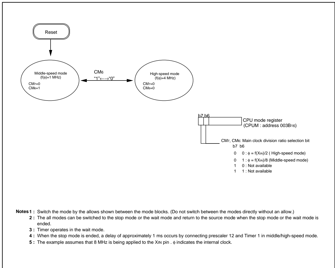
Fig. 45 State transitions of system clock
