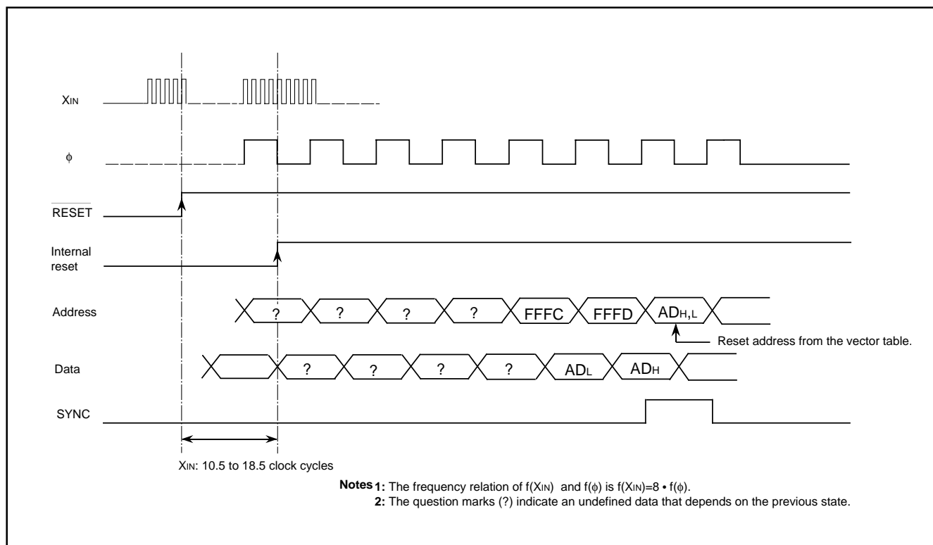
Fig. 40 Reset sequence
