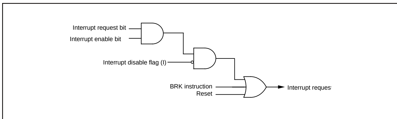
Fig. 26 Interrupt control
