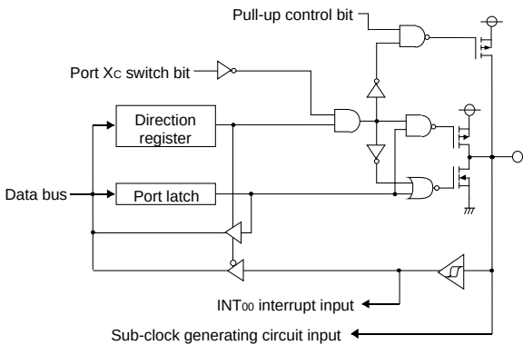
(11) Port P41
