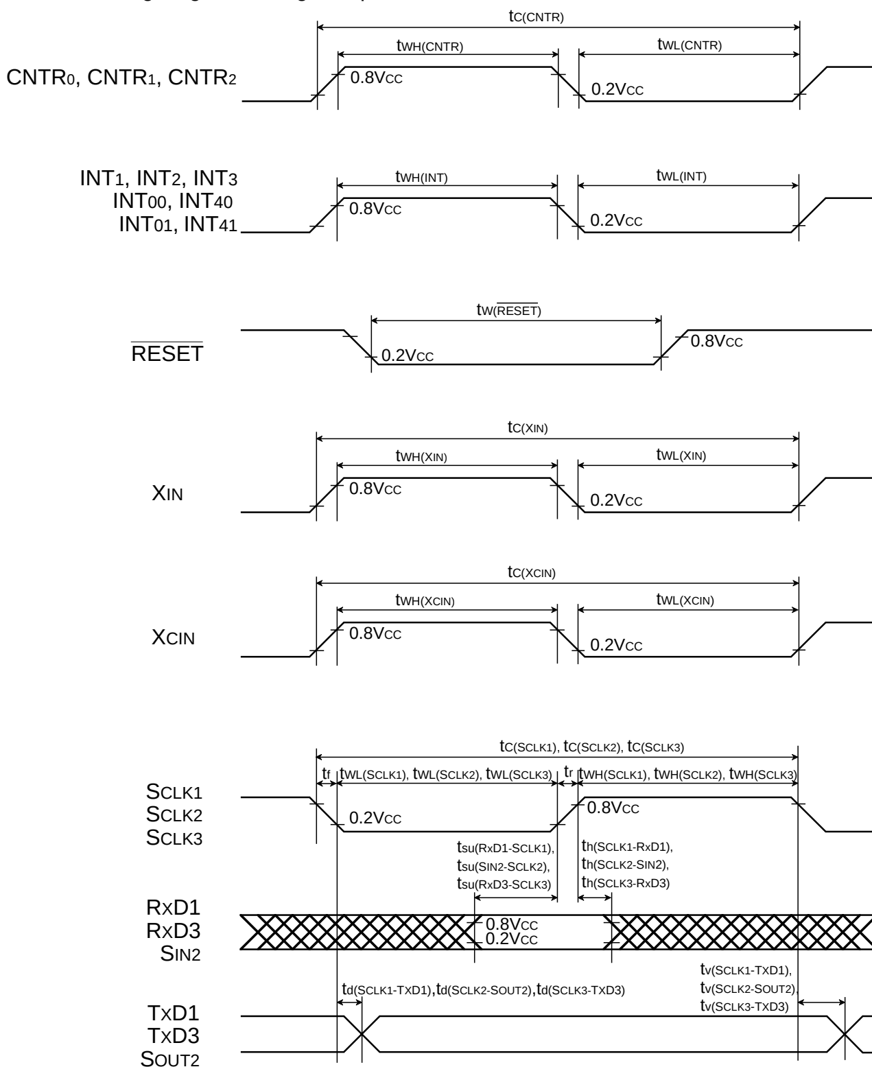
Fig. 107 Timing diagram (in single-chip mode)
