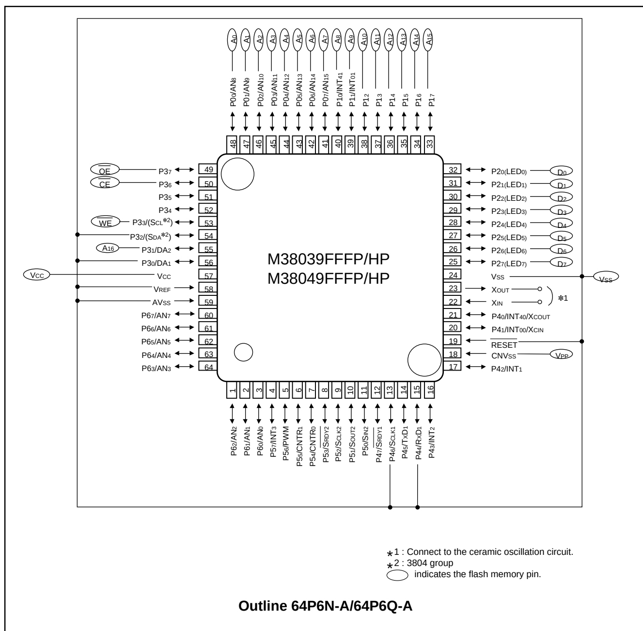
Fig. 86 Pin connection when operating in parallel input/output mode (M38039FFFP/HP, M38049FFFP/HP)
