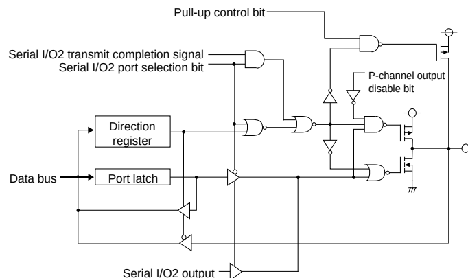
(14) Port P51
