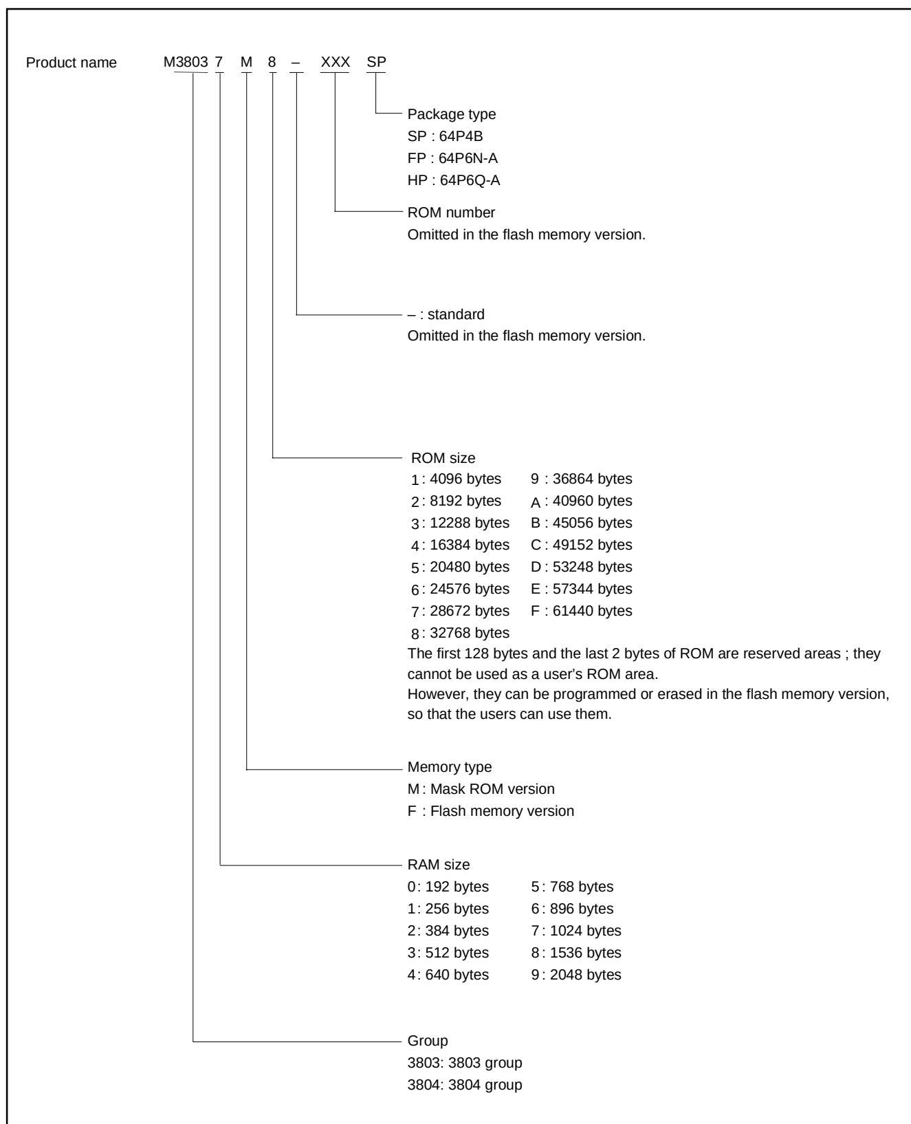
Fig. 7 Part numbering
