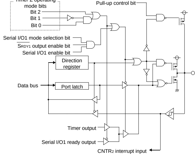
(14) Port P51
