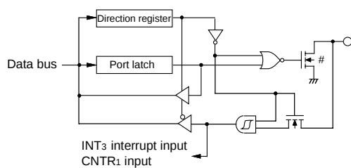
(8-1) Ports P45, P46
