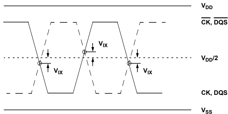
Figure 5. V_{IX} Definition
