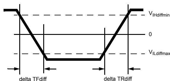
Figure 6. Differential Input Slew Rate definition for \overline{DQS} , \overline{DQS} and \overline{CK} , \overline{CK}
