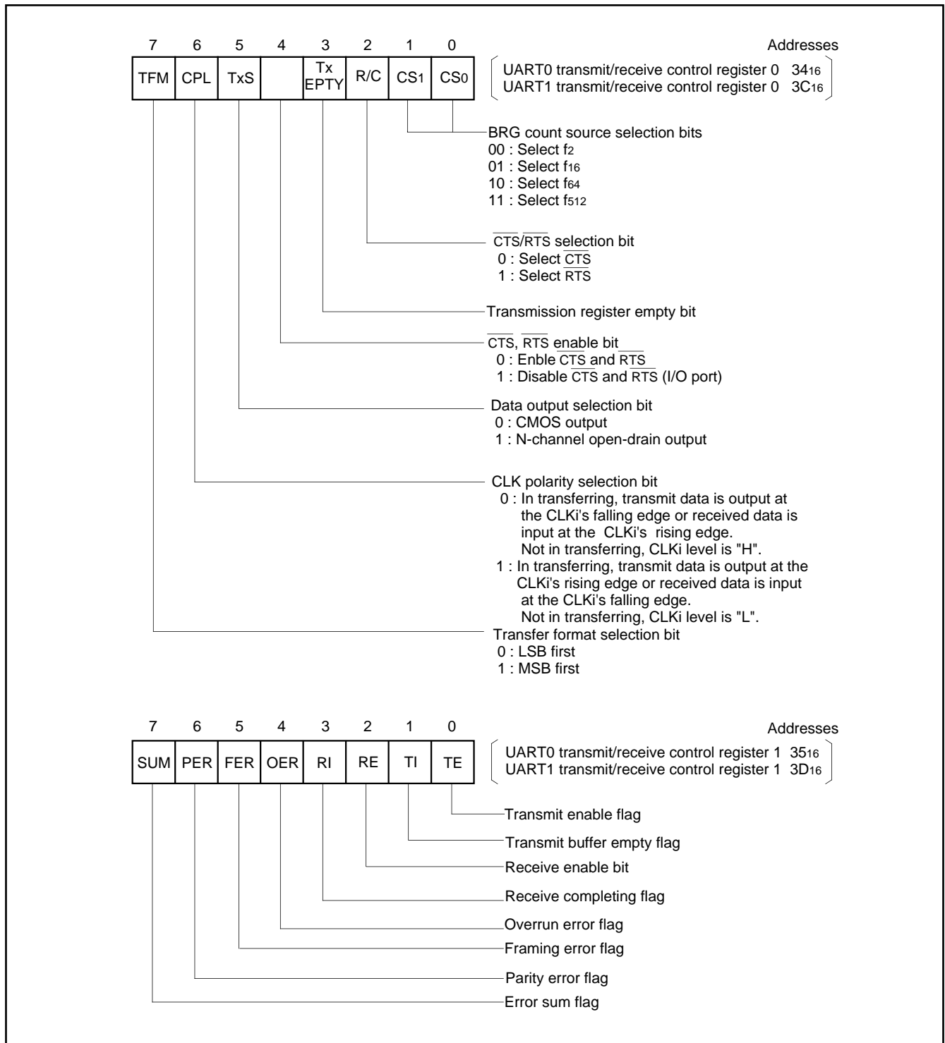
Fig. 39 UART0, UART1 transmit/receive control registers bit configuration
