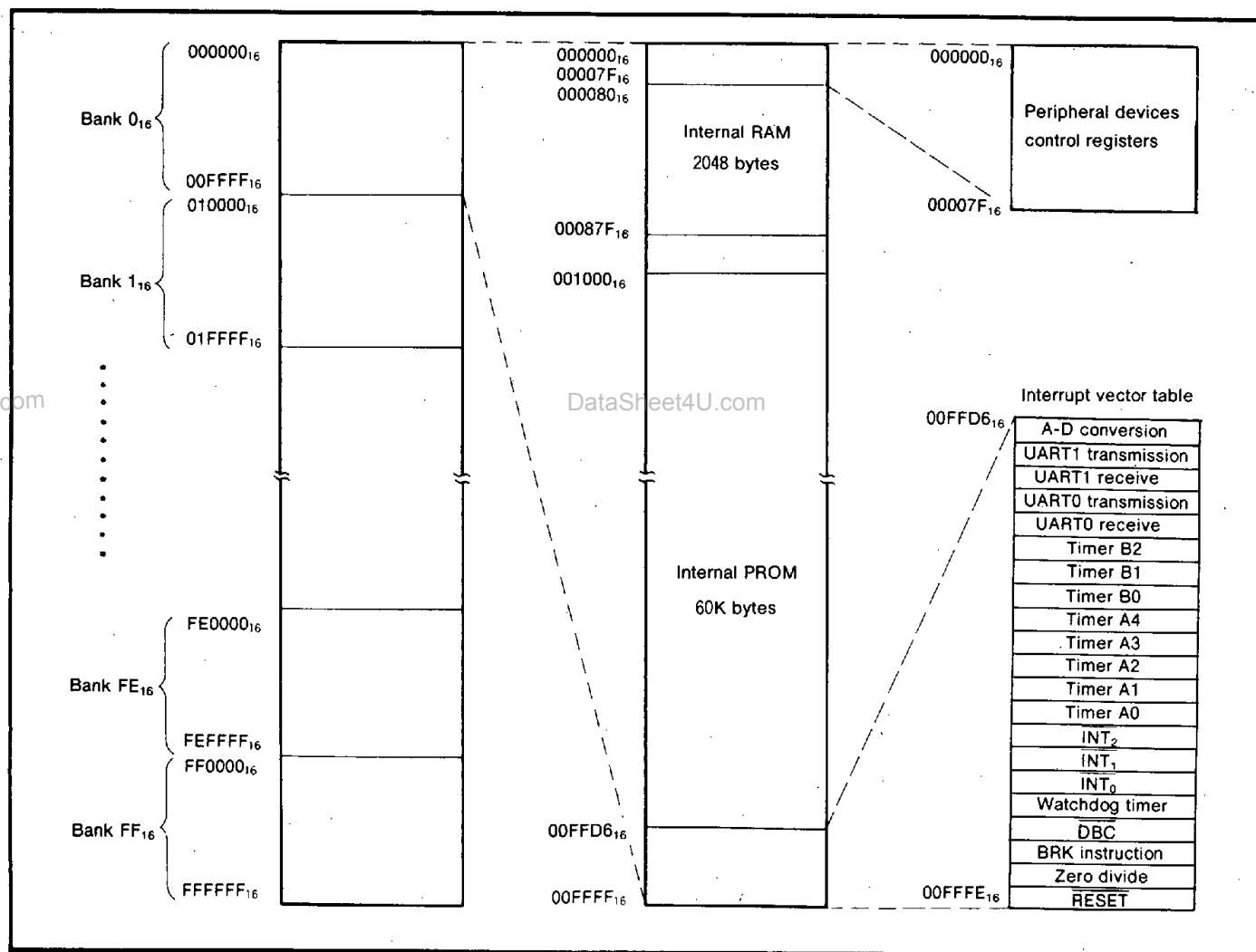
Fig. 1 Memory map
