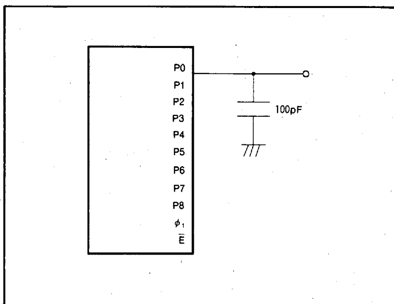
Fig. 3 Testing circuit for ports P0~P8, \phi_1
