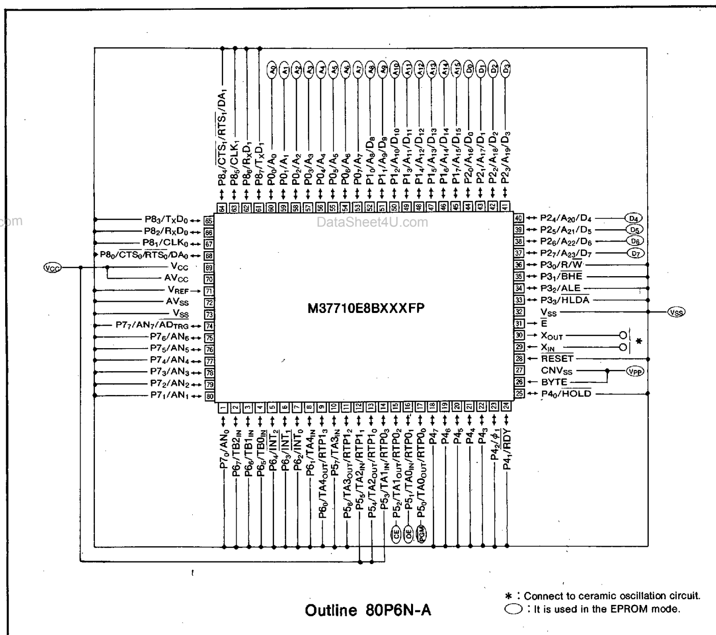
Fig. 2 Pin connection in EPROM mode
